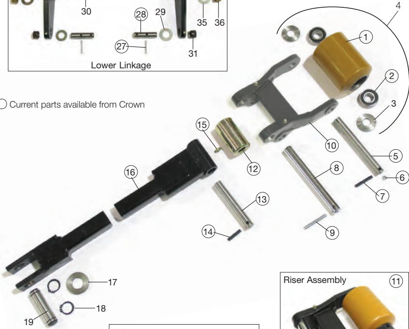
Upper Linkage
